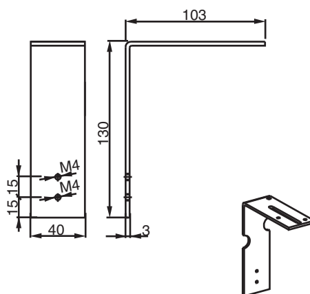
Z - Holder into Heluz 165 lintel
