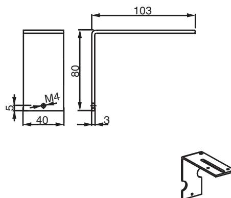
DK 567kp - 130 - Part for fixing the cover plate
