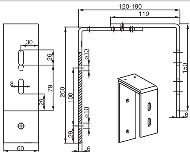
PPF 1 - Under-plaster holder – façade, sliding
