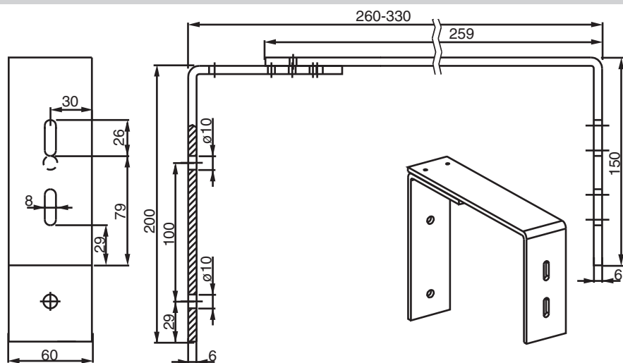
PPF 3 - Under-plaster holder – façade, sliding
