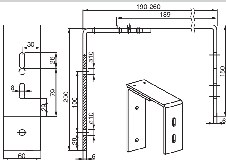
PPF 3 - Under-plaster holder – façade, sliding
