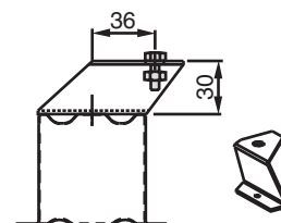
Z - Holder into Heluz 165 lintel
